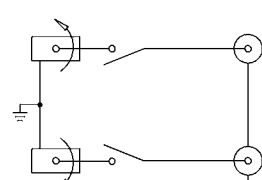
NON-NORMALLED NON-TERMINATED
