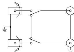
NORMALLED NON-TERMINATED
